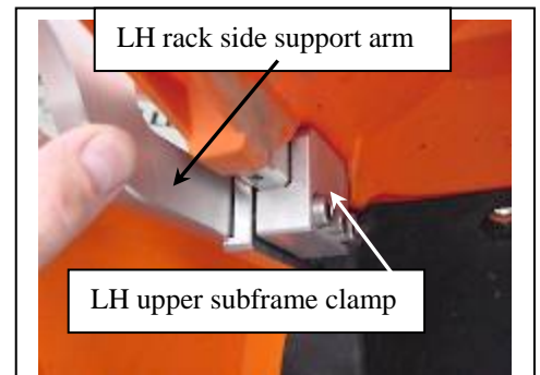
Figure 13: LH upper clamp and side arm install
